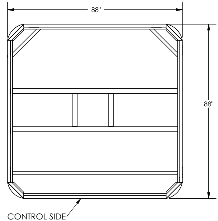
PLAN VIEW OF FOOTPRINT
