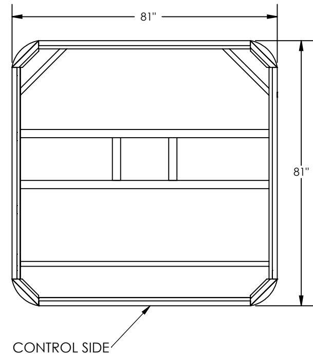
PLAN VIEW OF FOOTPRINT
