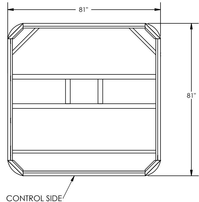
PLAN VIEW OF FOOTPRINT
