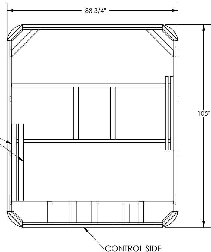
PLAN VIEW OF FOOTPRINT
