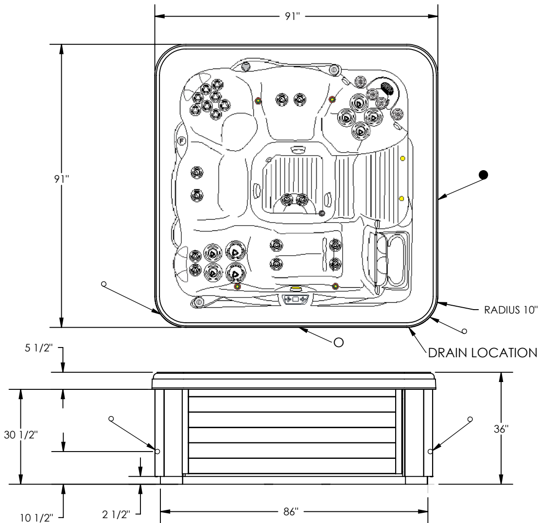
PLAN VIEW OF FOOTPRINT
