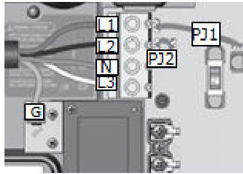
3-phase with single neutral
