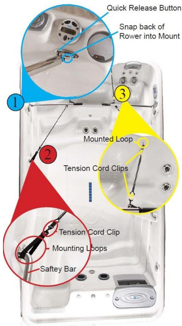
Figure 11. Rowing Equipment and Tension Cord Mount Locations
